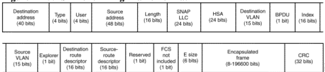
Figure A-15: ISL Token Ring Frame Format
